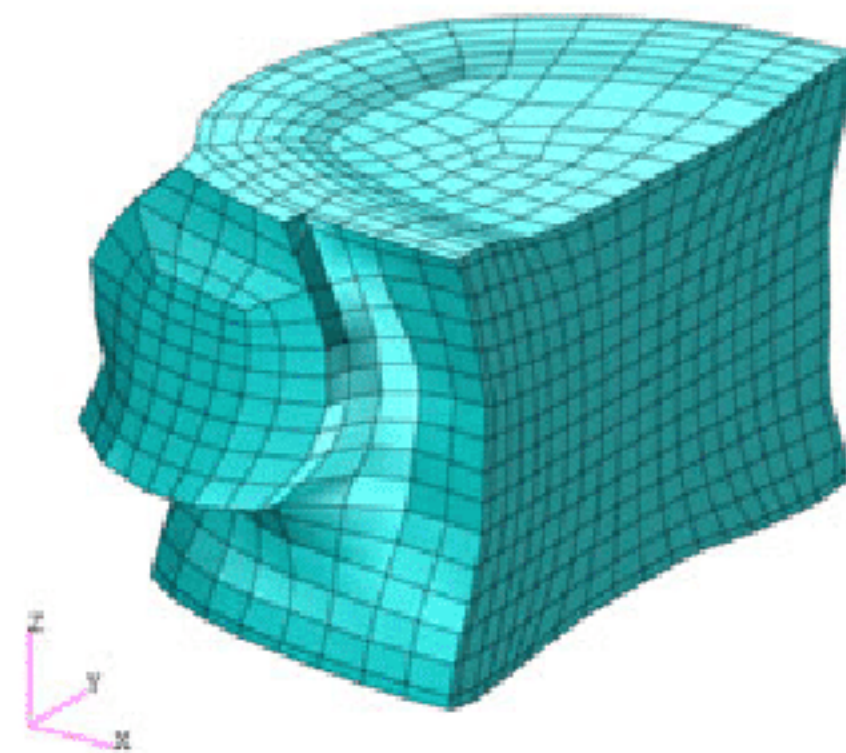
Original mesh
