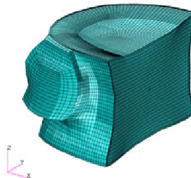
32 times refined mesh
